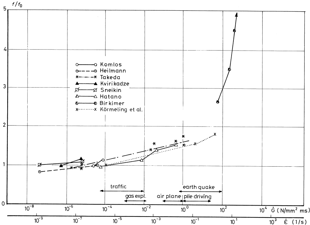
Fig. 1. Relative impact tensile strength as a function of loading rate.
