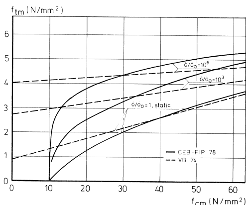
Fig. 23. Relation between concrete tensile strength and cube strength according to VB formulae (12) and CEB-FIP formulae (13) at three loading rates.
