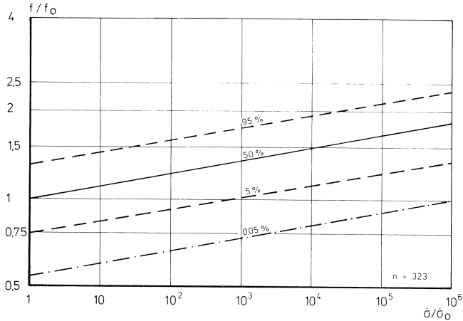
Fig. 7. Relative strength as a function of relative loading rate.
