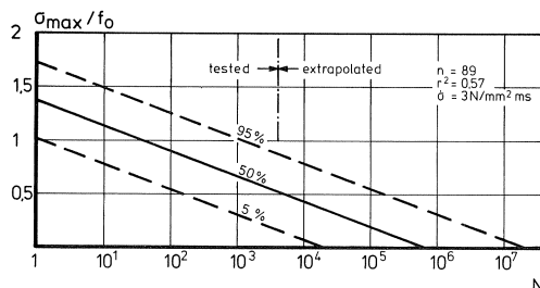
Fig. 11. Relation between relative maximum stress and the number of impact loads for all the results.
