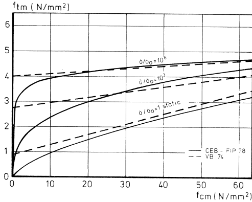
Fig. 25. Relation between concrete tensile strength and cube strength according to VB formulae (12) and modified CEB-FIP formulae (17) at three loading rates.
