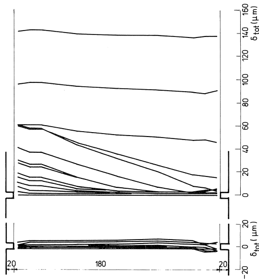
Fig. A4.5 Deformation distribution of the test of Fig. A4.4. Upper part: deformation at envelope stresses. Lower part: deformation at lower stress.
