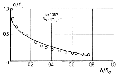
Fig. A5.2 Another example of an envelope curve with k=0,357 and \delta_0=175 \mu\text{m} .
