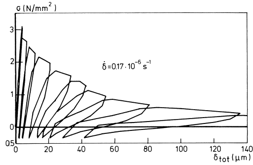
Fig. A4.2 Stress deformation curve of a test with a small compressive lower stress.
