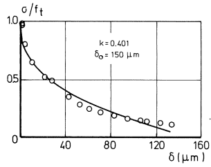
Fig. A5.1 Curve fitting of an envelope curve with k=0,401 and \delta_0=150 \mu\text{m} .
