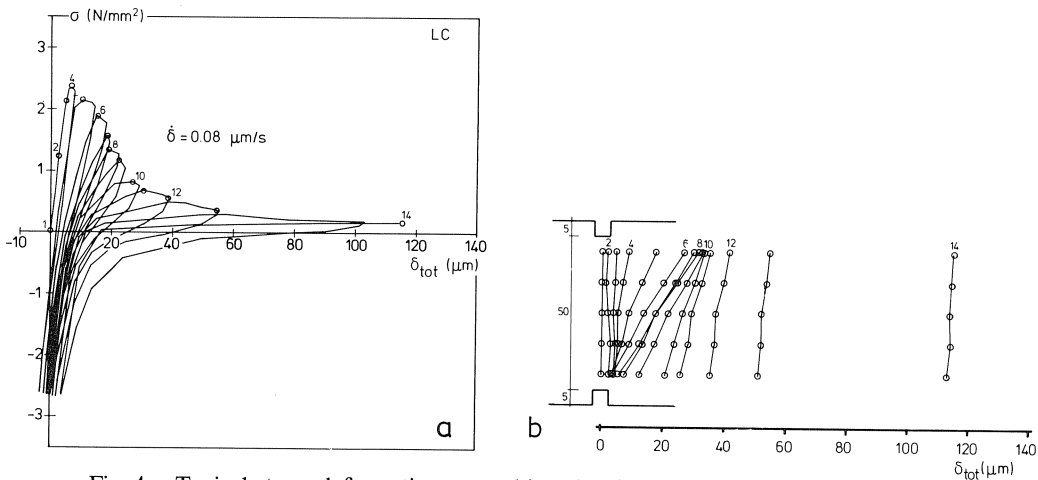
Fig. 4. Typical stress deformation curve (a) and deformation distribution for LC (b).
