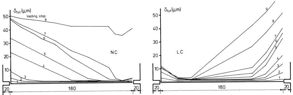
Fig. 10. Deformation distribution of wide NC and LC specimens.
