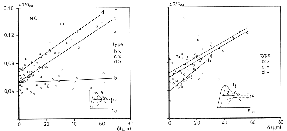
Fig. 8. Stress drop on the envelope curve after post-peak loading cycles.
