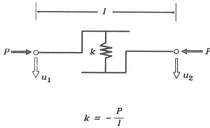
Figure V.4 P - \delta Spring with Deformation Change
