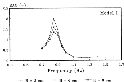
Figure 6.5 Measured RAOs for Deck Displacement with Different Wave Heights (Model I, Regular Waves)
