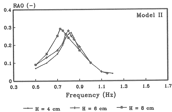
Figure 6.6 RAOs for Different Wave Heights (Model II, Regular Waves)
