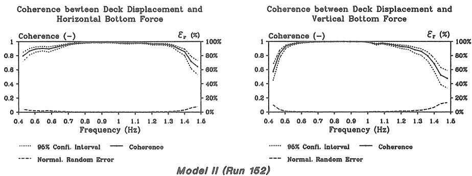
Figure 7.13 Coherence between Inter-Structural Quantities
