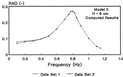
Figure 6.14 Comparison of Different Connecting Modeling
