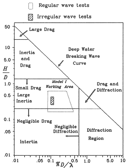
Figure III.4 Relative Importance Drag vs Inertia, Model I
