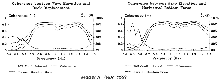
Figure 7.12 Coherence between Water-Related Quantity and Structure-Related Quantities
