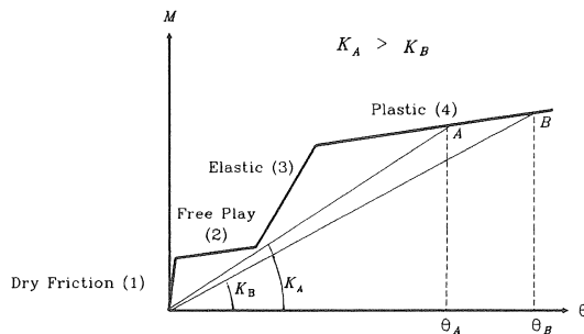
Figure II.3 Possible Deck-leg Connection Constitutive Relation
