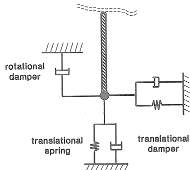
Figure V.5 Leg to Bottom Schematization
