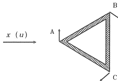
Figure I.4 Deck Displacement Caused by Rotation
