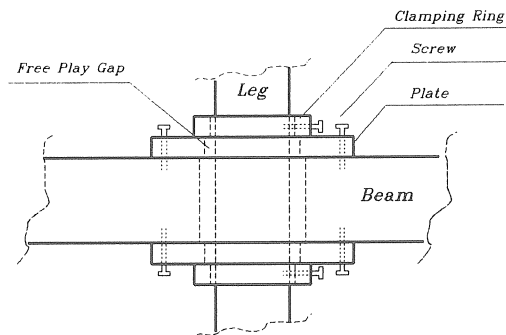
Figure II.2 Deck-leg Connection Detail
