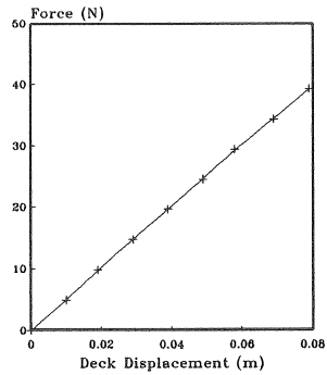
Figure 3.2 Measured Overall Static Constitutive Relation (Model I)
