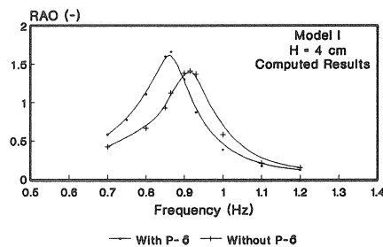
Figure 6.16 Influence of P-\delta Effect
