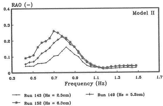
Figure 7.9 RAOs for Different Wave Heights (Model II, Irregular Waves)
