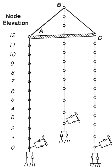
Figure 6.4 Schematization for Model II in Air
