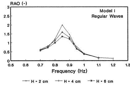
Figure 6.10 Measured RAOs for Various Wave Heights (Model I, Regular waves)
