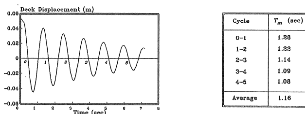
Figure II.1 Free Vibration Response Record
