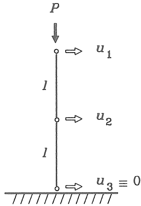
Figure IV.3 Applicability of P- \delta Elements
