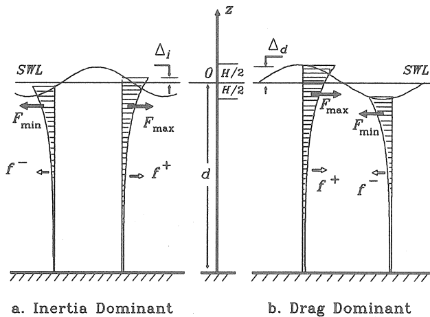
Figure IV.1 Hydrodynamic Force Skewness
