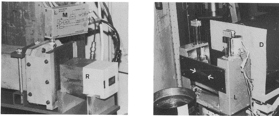
Fig. 2. On the left-hand side view of monitor (M) and restriction (R). On the right-hand side view of lift (L) with front diaphragm (see arrows) and detector (D).
