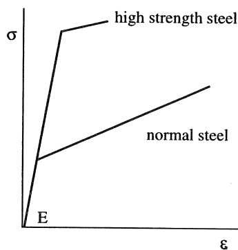
Fig. 3. \sigma - \epsilon diagrams for various material properties.
