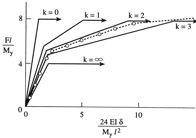
Fig. 2. Load deflection relations for beam of figure 1 (from [11]) (dotted line indicates test results).
