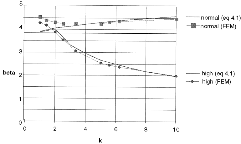
Fig. 4. Reliability index \beta for normal and high strength steel as a function of k ( kl = side span length); FEM and simplified calculation
