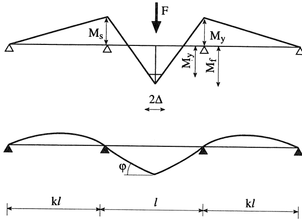
Fig. 6. Moments and displacements.
