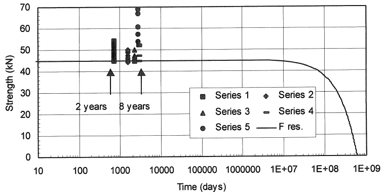
Fig. 5.1 Development of the average load carrying capacity of nailed joints.
