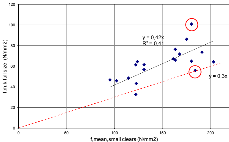
Figure 8. Relation between the mean value of small clear samples of cumaru and the 5%-values derived from full size specimens of the same timber species
