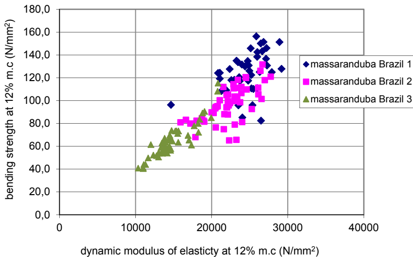
Figure 9. Relation between the dynamic modulus of elasticity and the bending strength for all specimen of the three massaranduba samples
