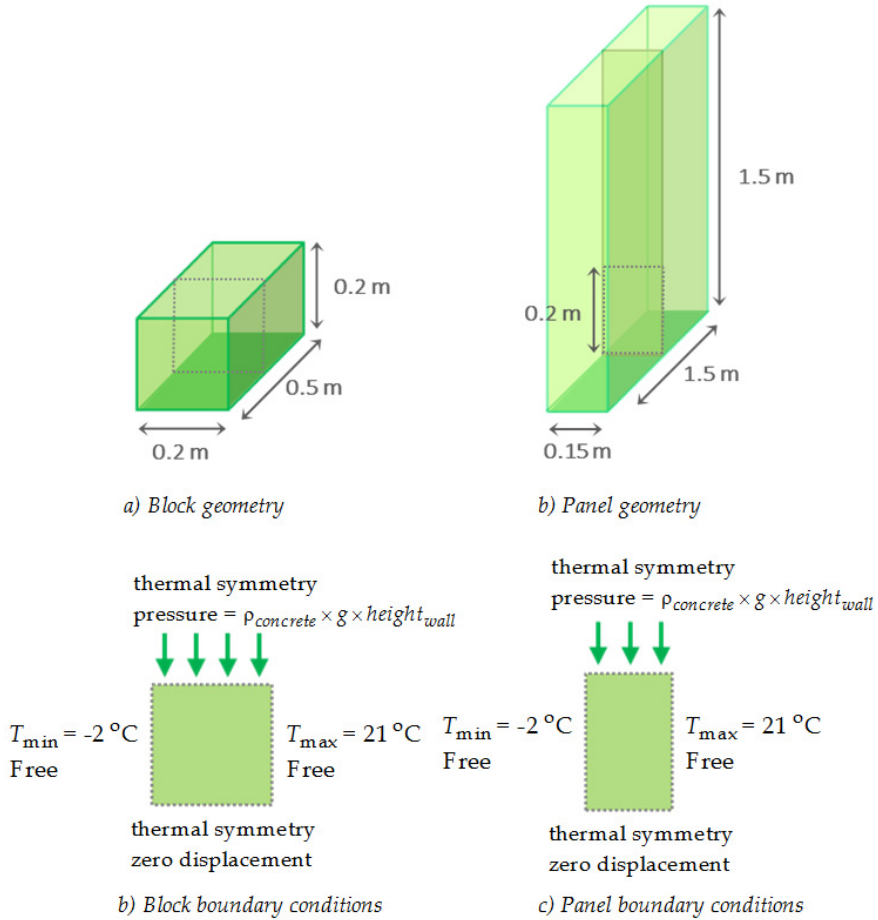
Figure 1: 2D Geometries of simulation domains and corresponding mechanical and thermal boundary conditions (BC) (height wall is 2.7 m for blocks made wall and 3 m for panels made wall)
