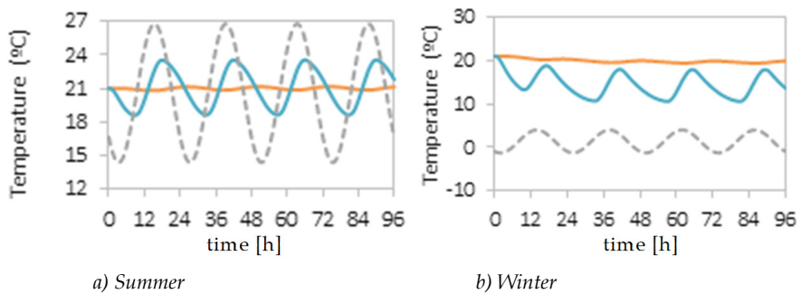
Figure 5: Temperature in the interior surface of walls as a function of time for each concrete mixture — interior wall surface Mix 2, — interior wall surface Mix 4, --- outdoor ambient temperature
