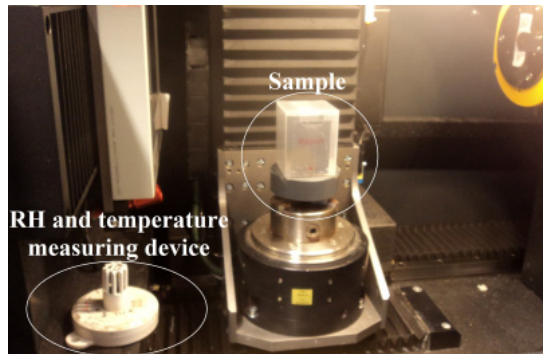
X-ray absorption setup with the position of the plastic container (sample) and sensor for temperature and relative humidity (RH)
